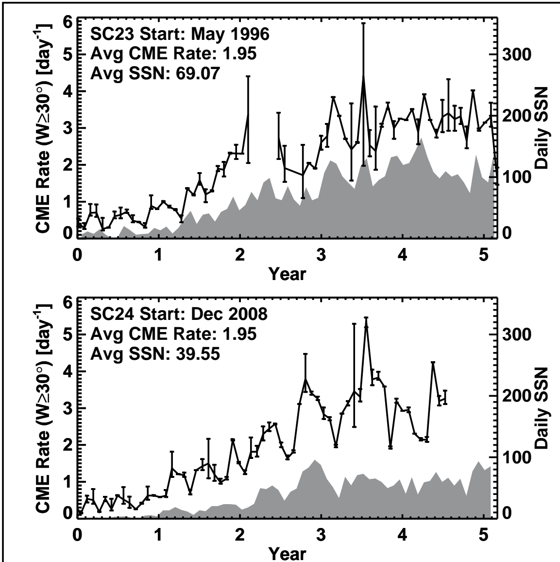
Figure 1. CME daily rate averaged over Carrington Rotation (CR) period (27.24 days). The error bars are derived from the cumulative down time in a given CR, counting data gaps (due to roll maneuver and LASCO electronics box anomalies) longer than 3 h. The upper limit was obtained assuming that during the downtime, CMEs occurred at the maximum daily rate of the CR. The lower limit was obtained assuming that no new CMEs occurred during the downtime. The plot in gray is the daily international sunspot number (SSN) obtained from Solar Influences Data Center ( http://sidc.oma.be/sunspot-data/ ). For definitiveness, we have included only CMEs with the width ( W ) \geq 30^\circ . This will eliminate the uncertainty due to narrow CMEs from the disk center missed by the coronagraph. Cycles 23 and 24 overlapped during the year 2008. CME measurements are not yet available after July 2013.
