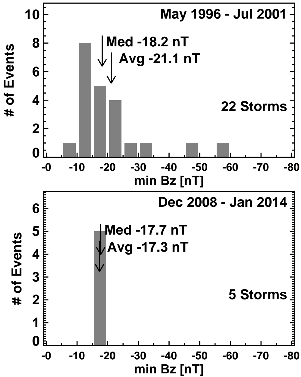
Figure 4. Distribution of B_z in major storms of cycle 23 (top) and cycle 24 (bottom).
