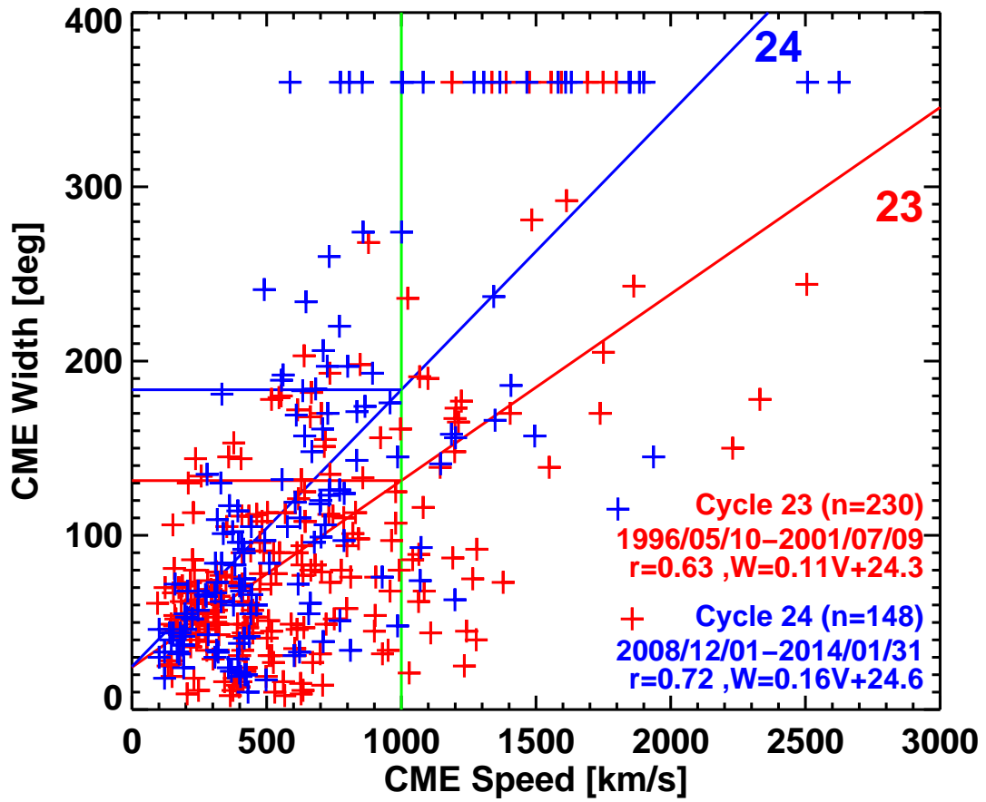
Figure 2. Scatterplots between CME speed (V) and angular width (W) for cycles 23 (red) and 24 (blue). The regression lines and the correlation coefficients are indicated on the plot. The width difference at 1000 km/s (green line) is substantial between the two cycles.
